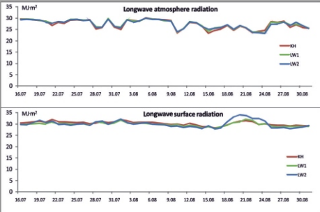
Course of longwave radiation in the Kaffiøyra region in the period 16.07-31.08.2010
