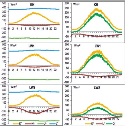
Average course of balance radiation fluxes and surface radiation balance ( Q^* ), net short wave radiation ( K^* ) and net long wave radiation ( L^* ) in the Kaffiøyra region in the period 16.07-31.08.2010
