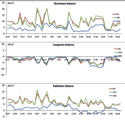
Course of net shortwave radiation and net longwave radiation and surface radiation balances in the Kaffiøyra region in the period 16.07-31.08.2010
