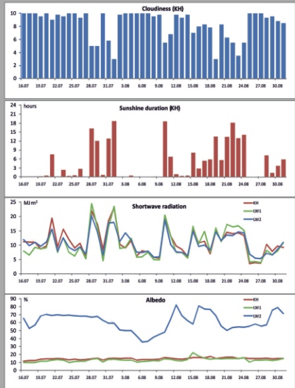
Course of cloudiness (B10) and sunshine duration (hours) at the KH stand and daily sums of short solar radiation ( MJm^{-2} ) and albedo at the stands: KH, LW1, LW2 in the period 16.07-31.08.2010
